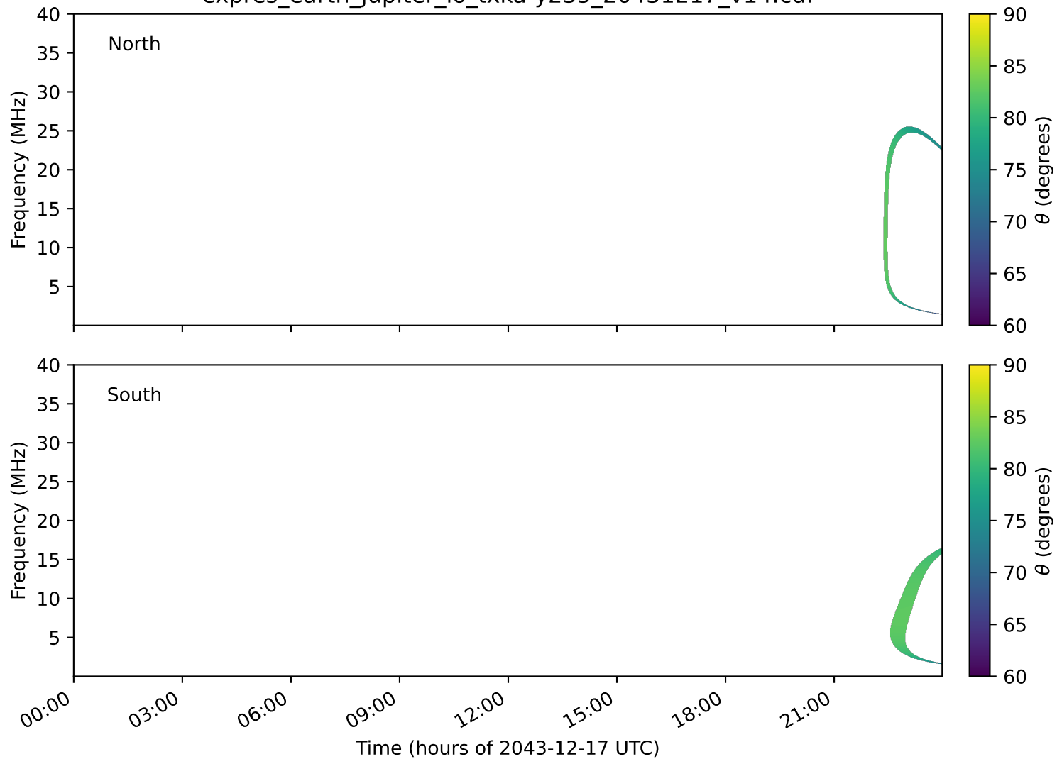
expres_earth_jupiter_io_txka-y235_20431217_v14.cdf
