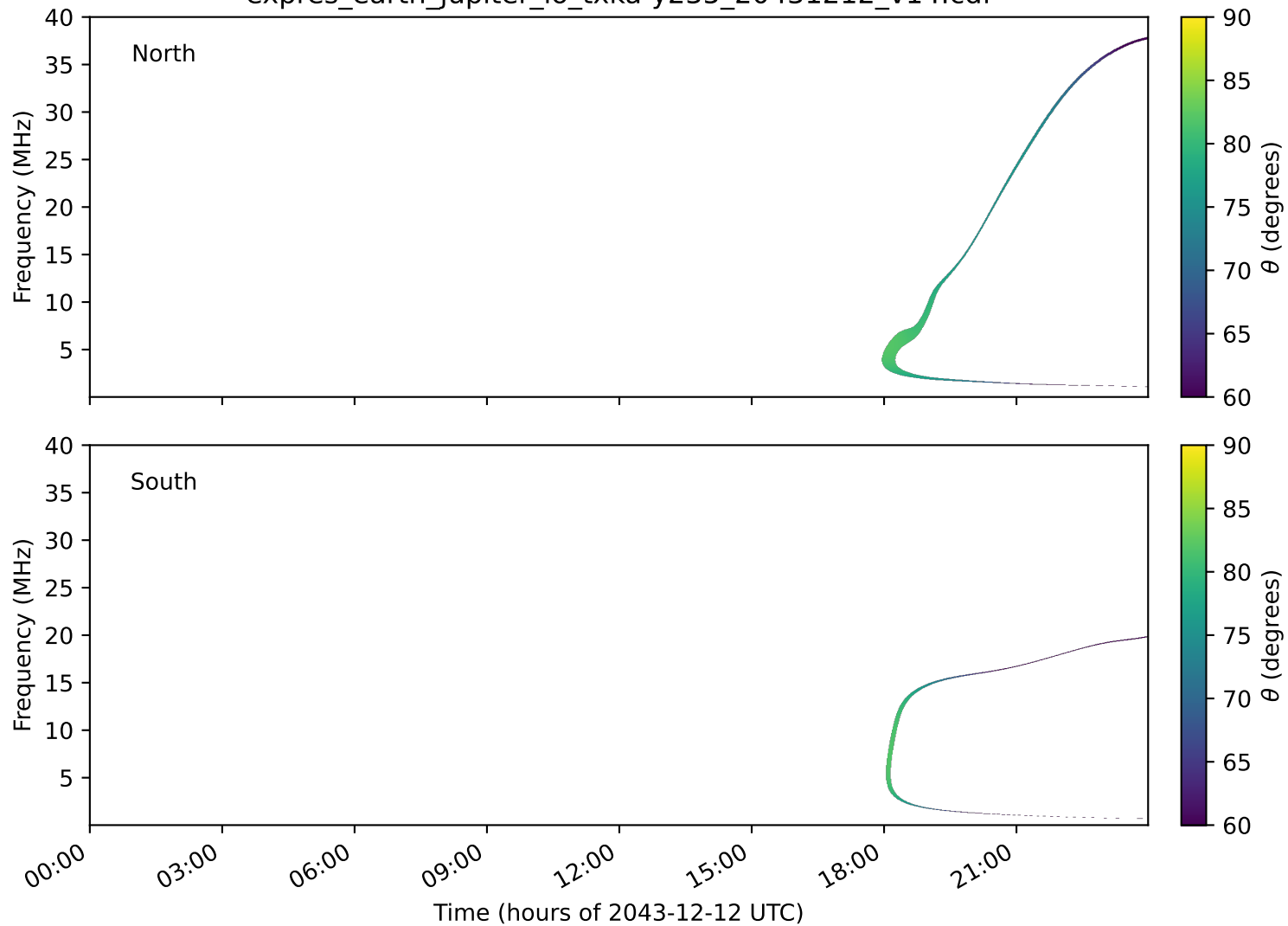
expres_earth_jupiter_io_txka-y235_20431212_v14.cdf
