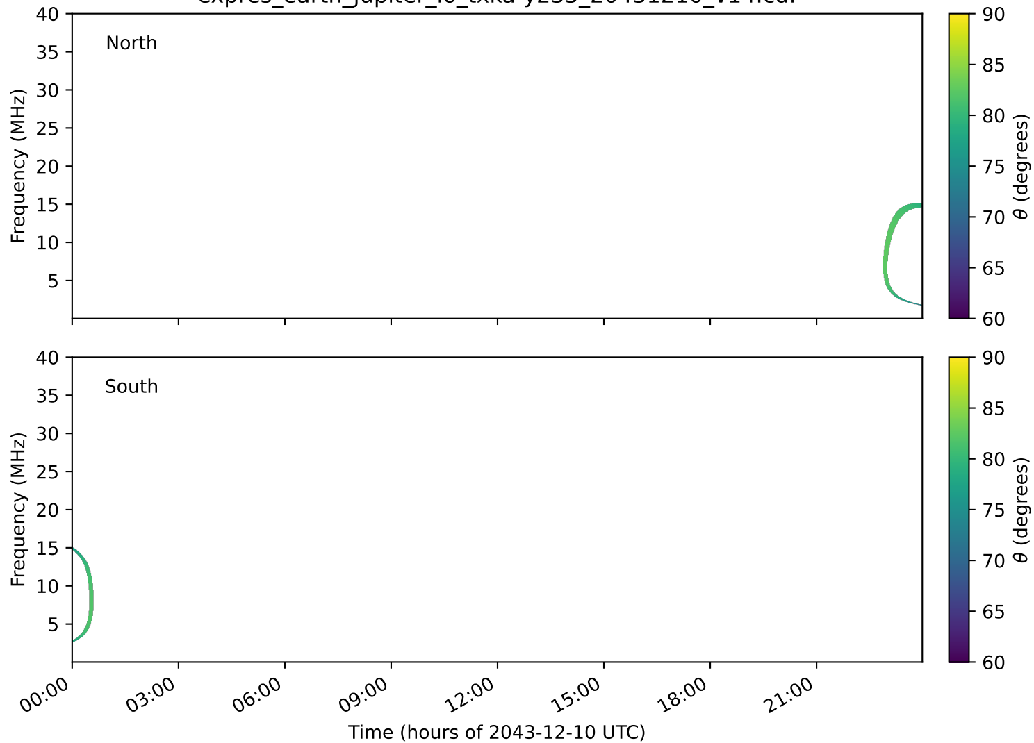
expres_earth_jupiter_io_txka-y235_20431210_v14.cdf
