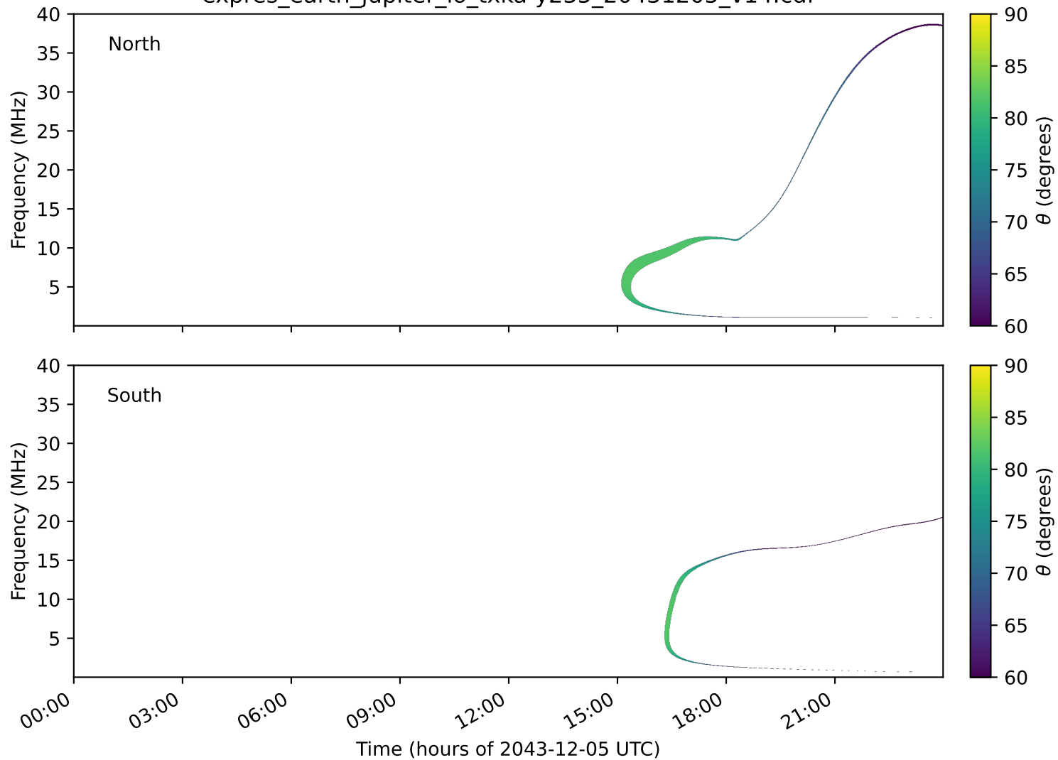
expres_earth_jupiter_io_txka-y235_20431205_v14.cdf
