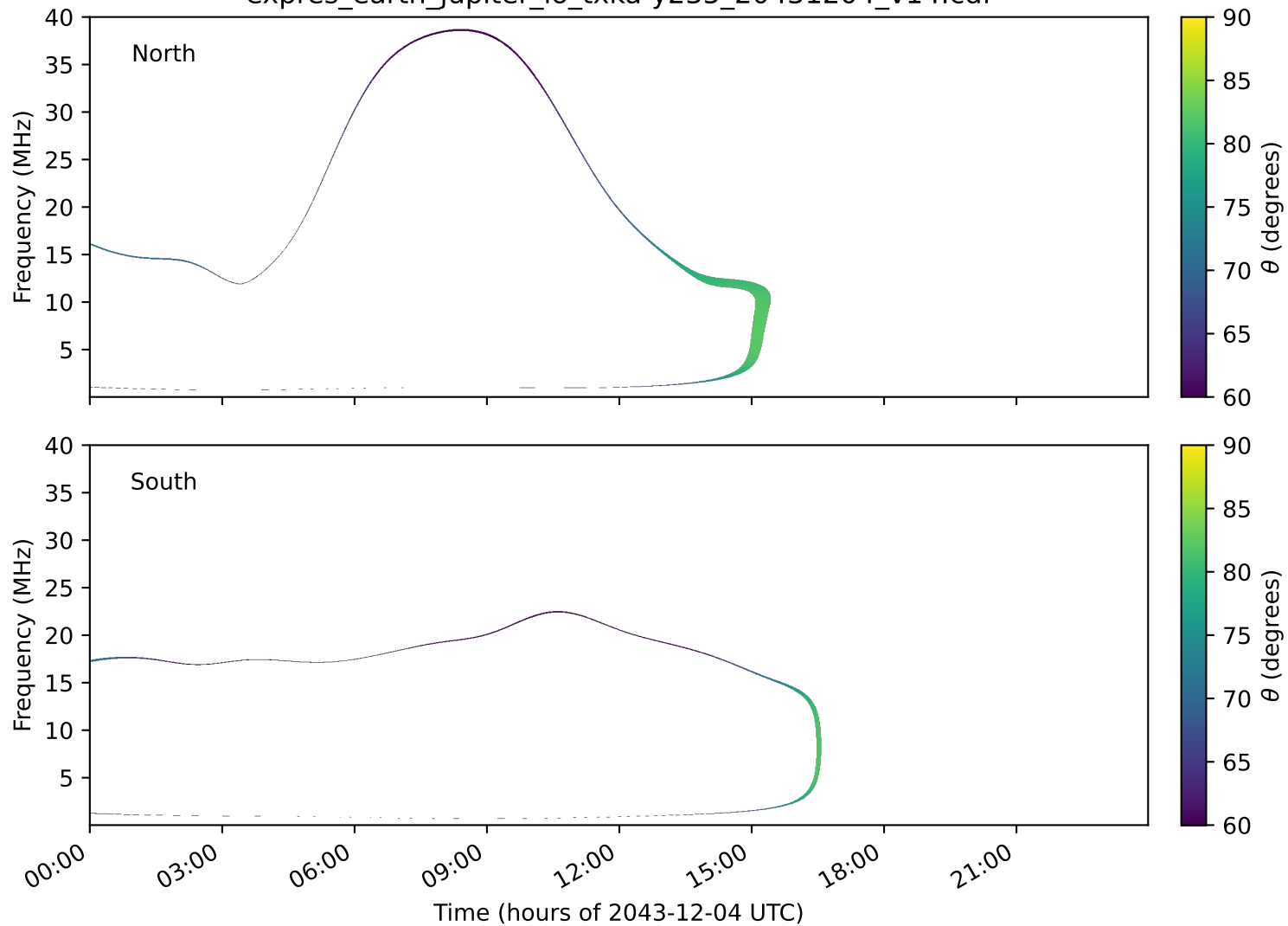
expres_earth_jupiter_io_txka-y235_20431204_v14.cdf
