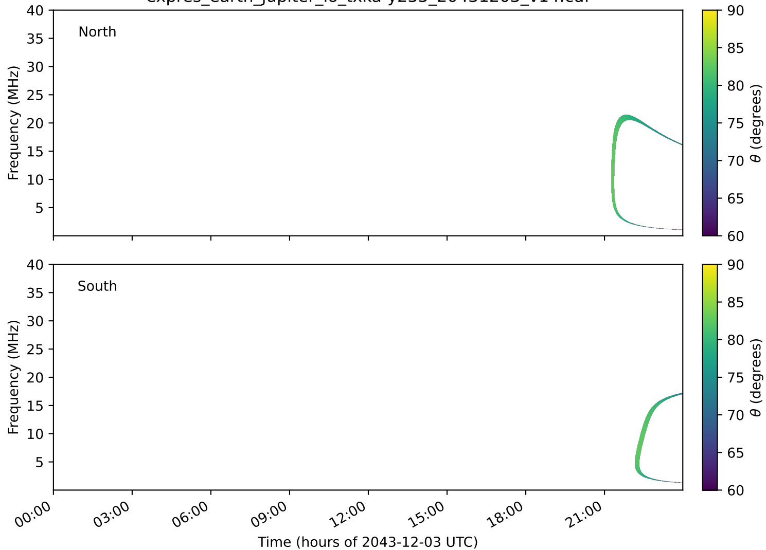
expres_earth_jupiter_io_txka-y235_20431203_v14.cdf
