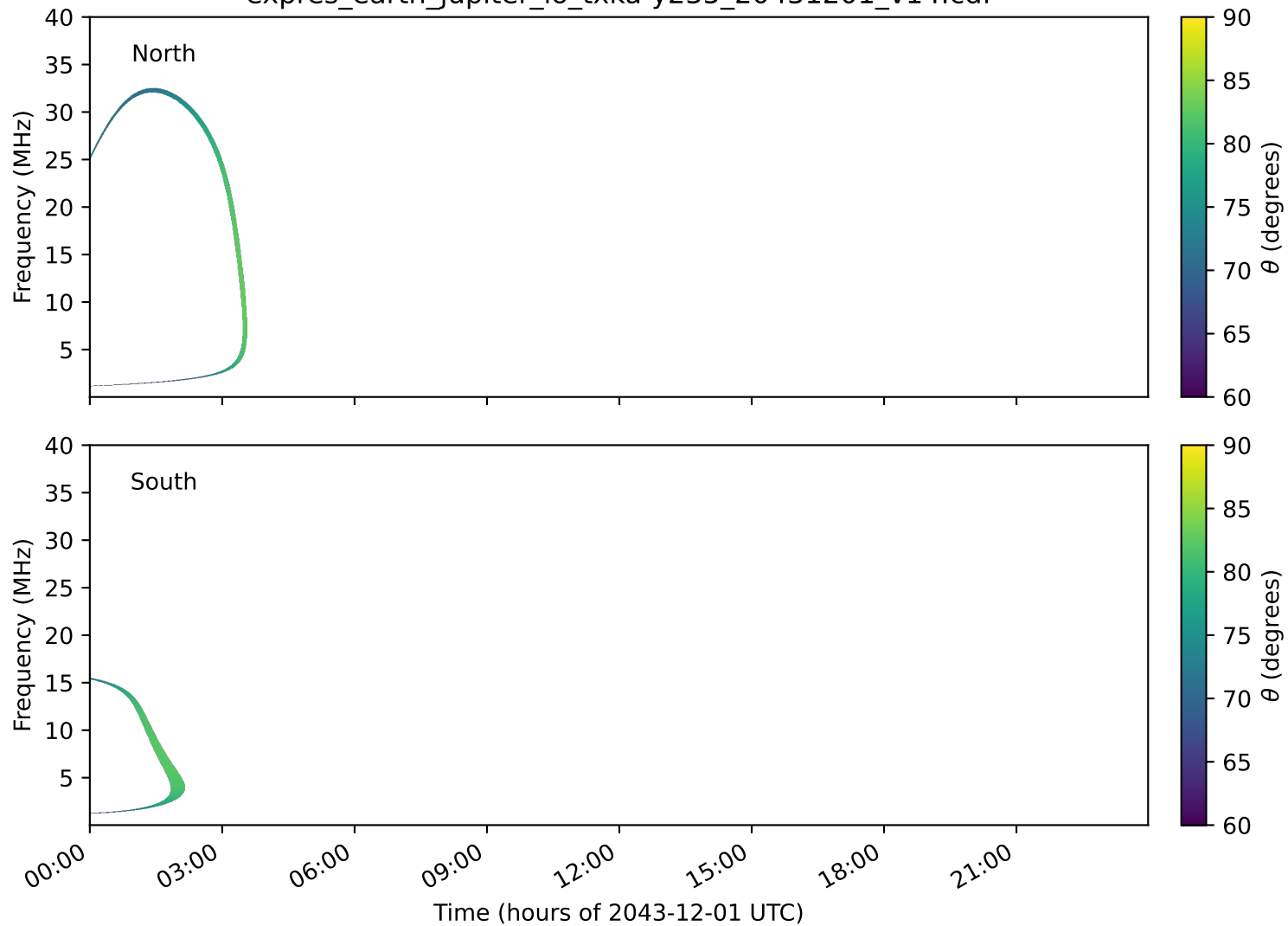
expres_earth_jupiter_io_txka-y235_20431201_v14.cdf
