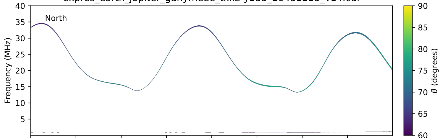
expres_earth_jupiter_ganymede_txka-y235_20431225_v14.cdf
