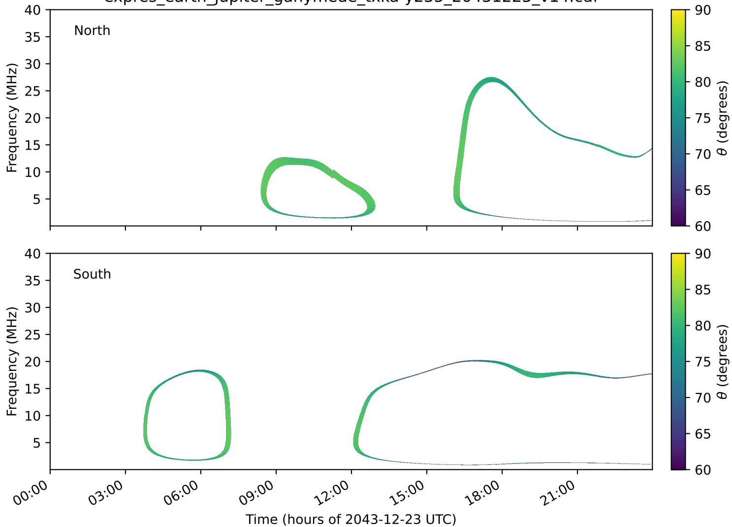
expres_earth_jupiter_ganymede_txka-y235_20431223_v14.cdf
