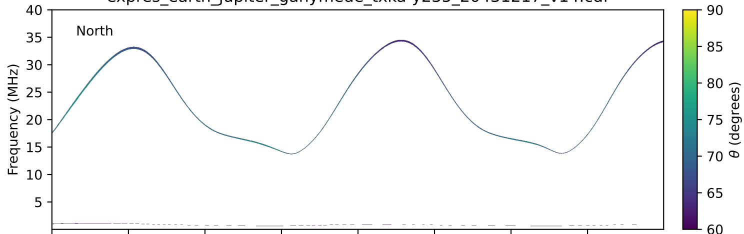
expres_earth_jupiter_ganymede_txka-y235_20431217_v14.cdf
