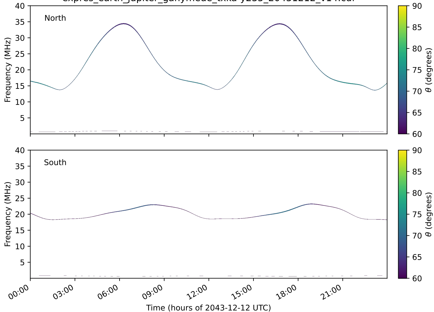
expres_earth_jupiter_ganymede_txka-y235_20431212_v14.cdf
