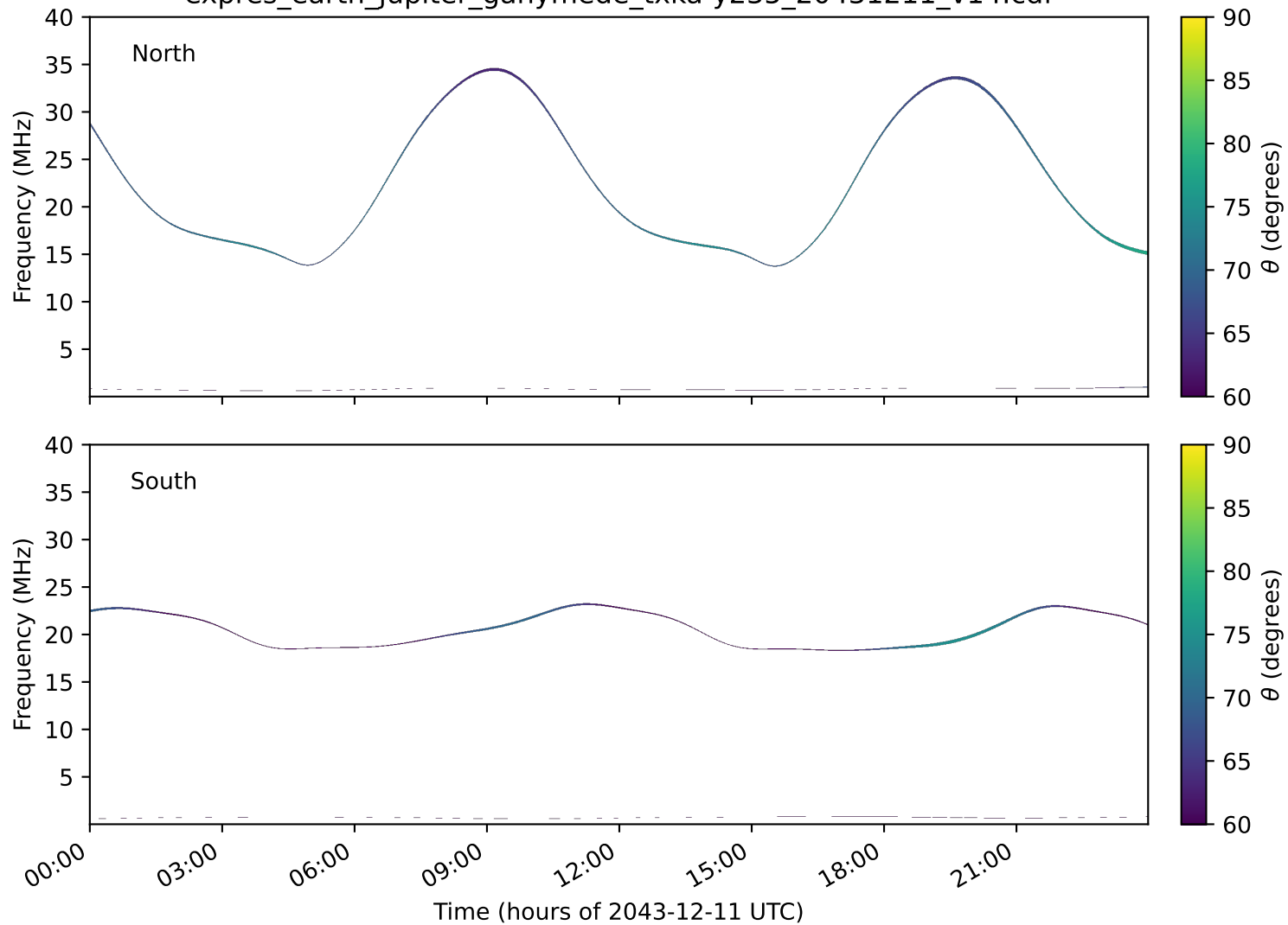
expres_earth_jupiter_ganymede_txka-y235_20431211_v14.cdf
