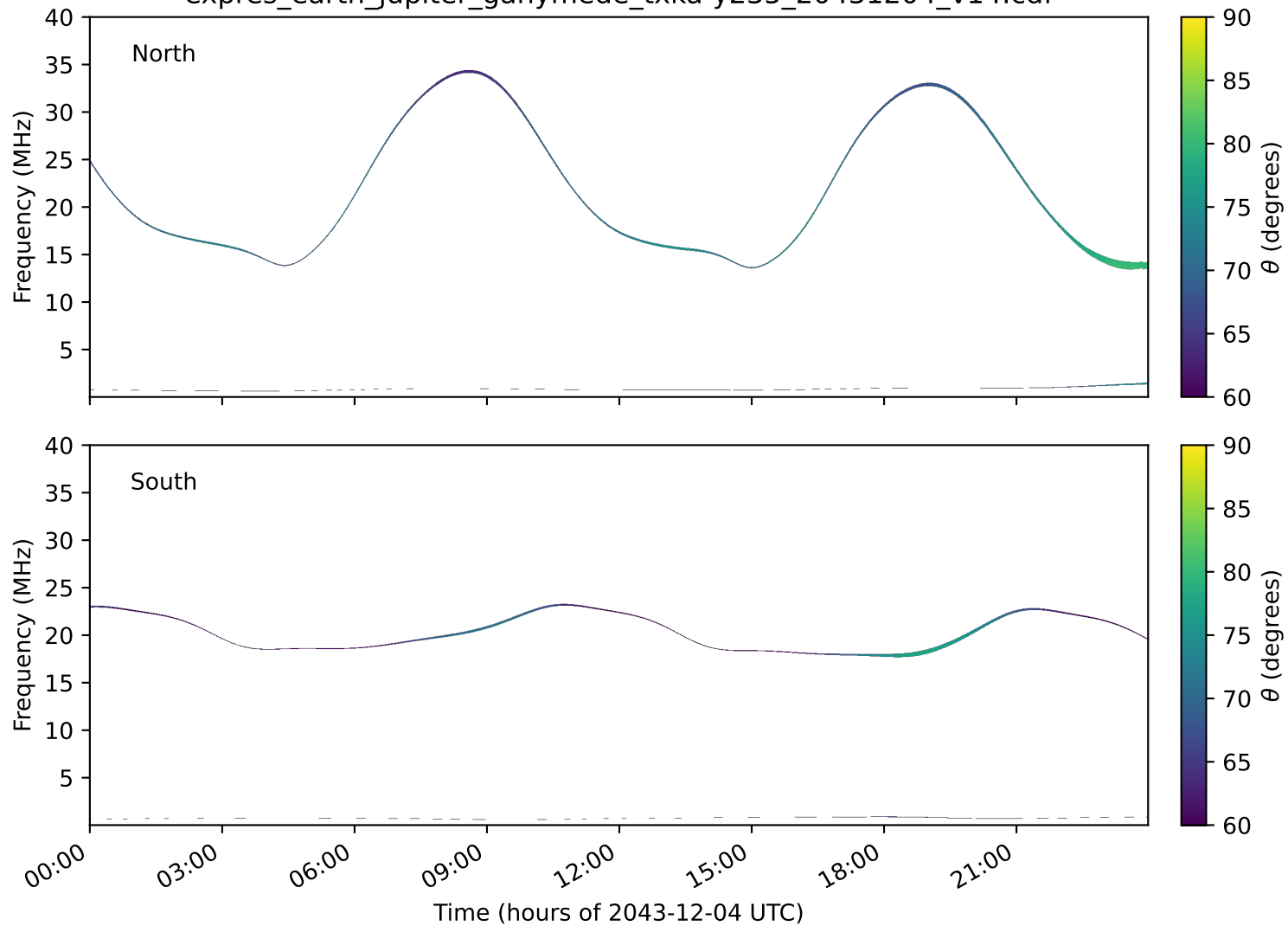
expres_earth_jupiter_ganymede_txka-y235_20431204_v14.cdf
