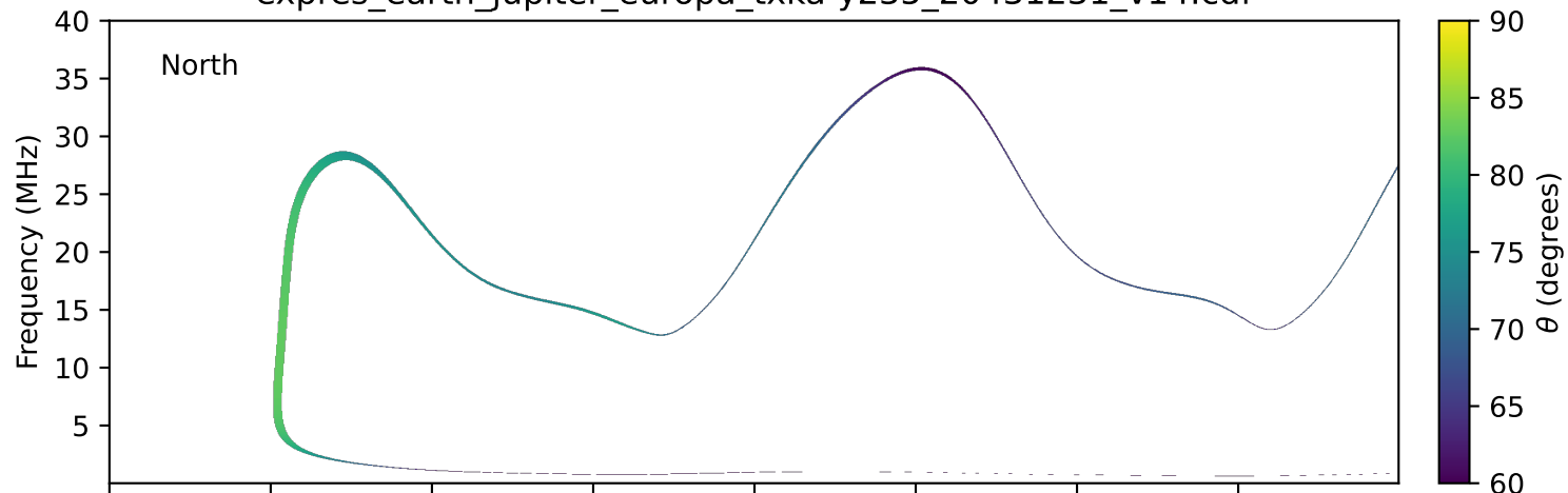
expres_earth_jupiter_europa_txka-y235_20431231_v14.cdf
