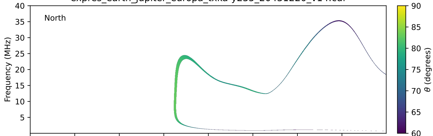
expres_earth_jupiter_europa_txka-y235_20431220_v14.cdf
