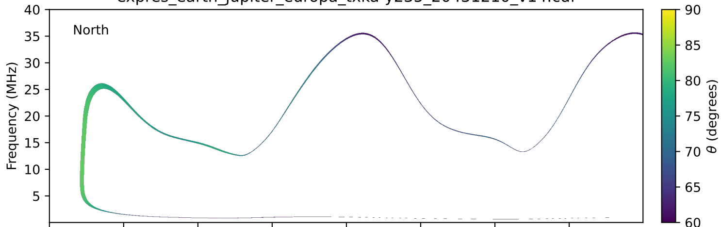
expres_earth_jupiter_europa_txka-y235_20431210_v14.cdf
