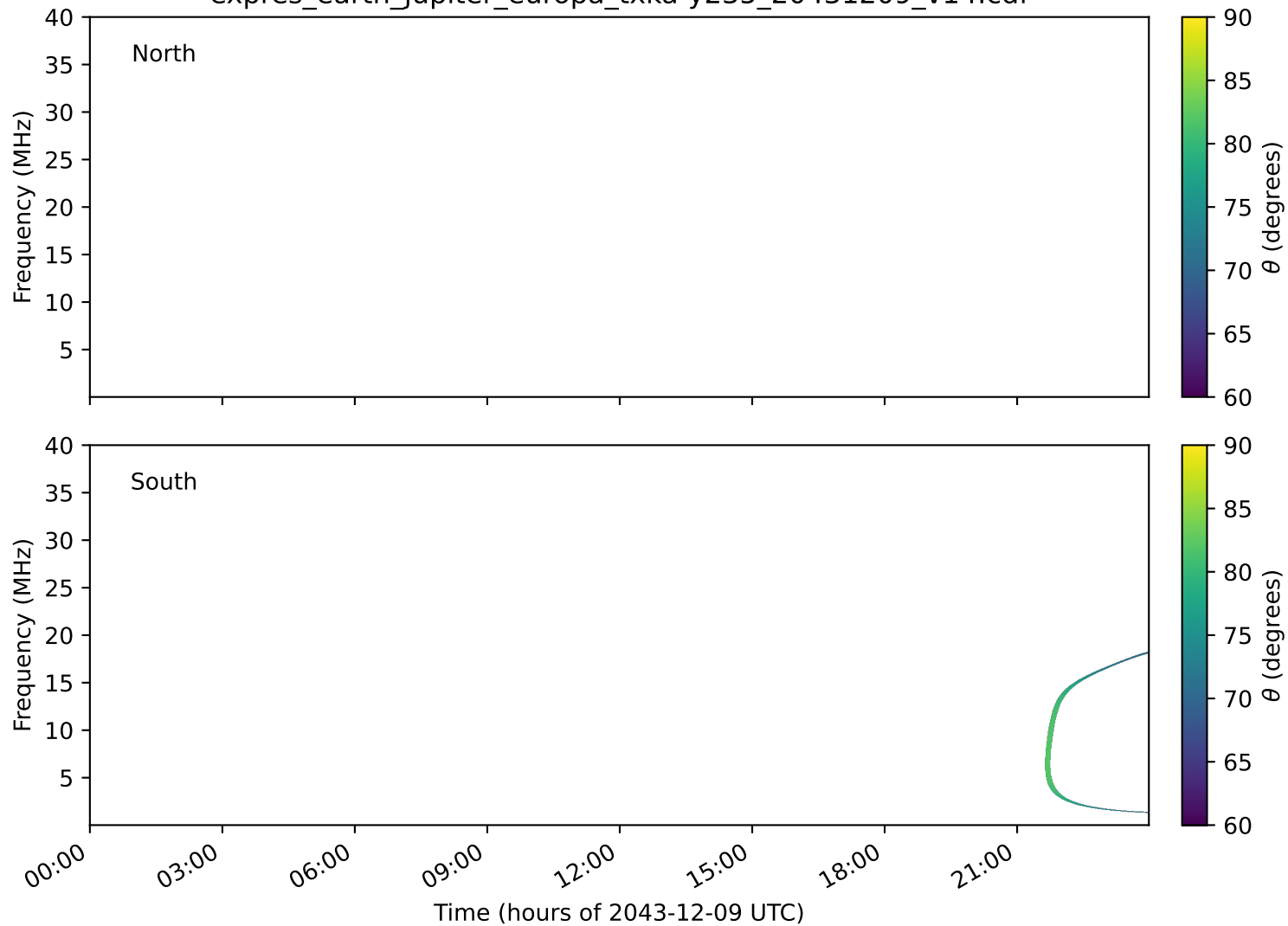
expres_earth_jupiter_europa_txka-y235_20431209_v14.cdf
