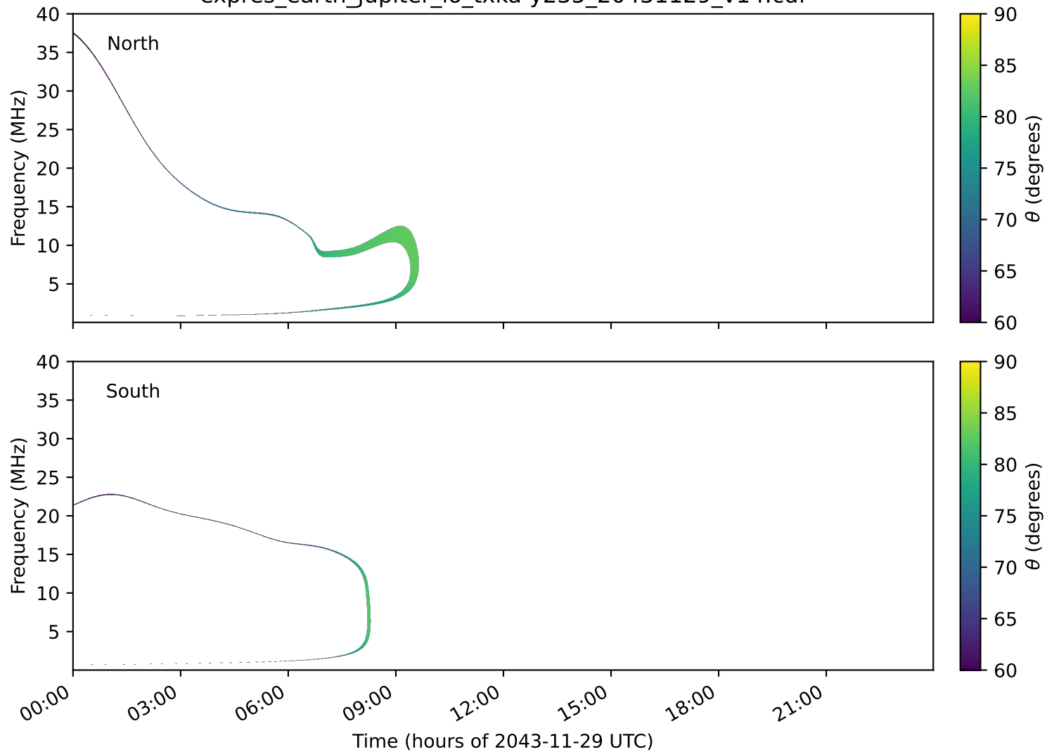
expres_earth_jupiter_io_txka-y235_20431129_v14.cdf
