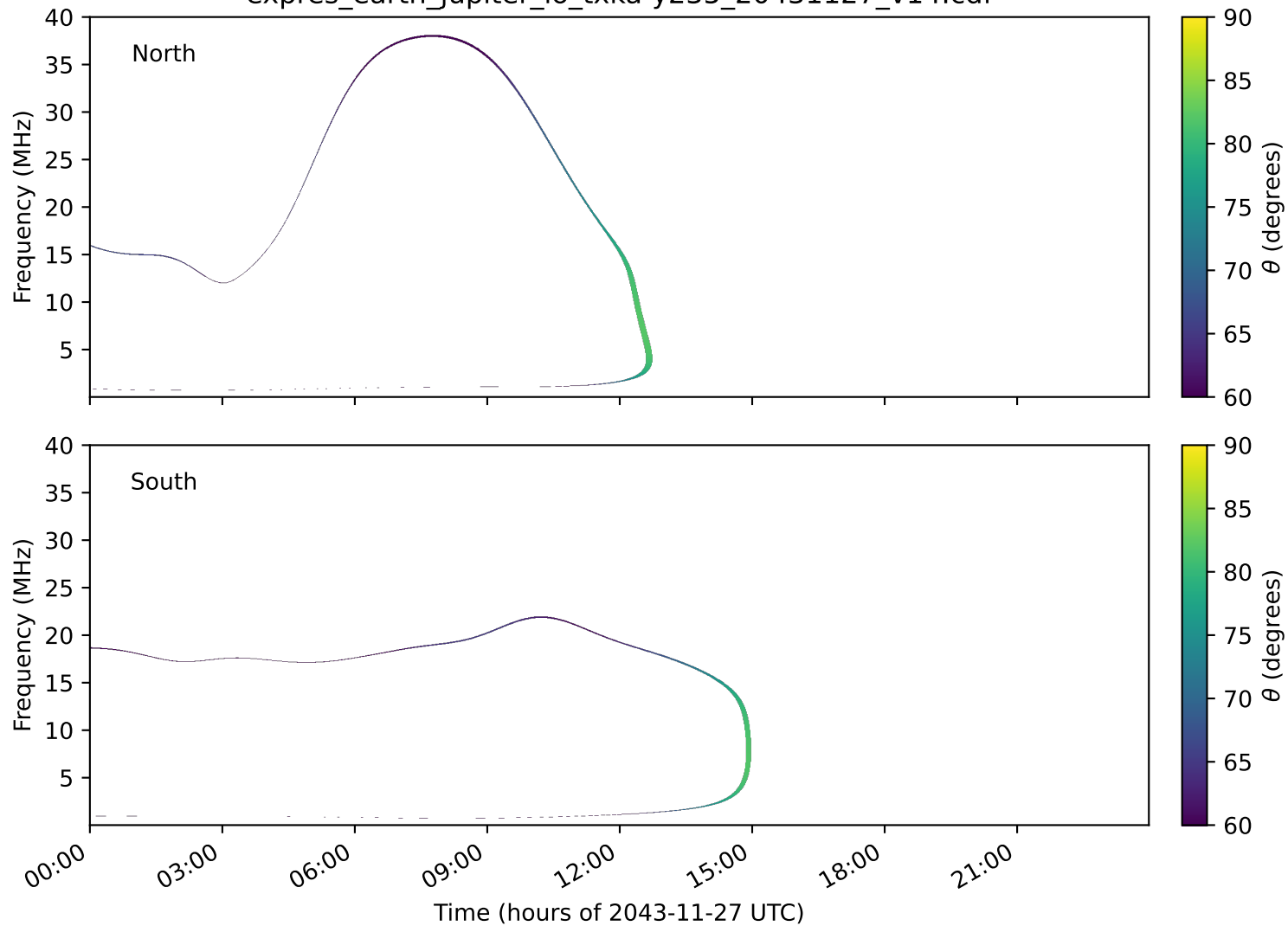
expres_earth_jupiter_io_txka-y235_20431127_v14.cdf
