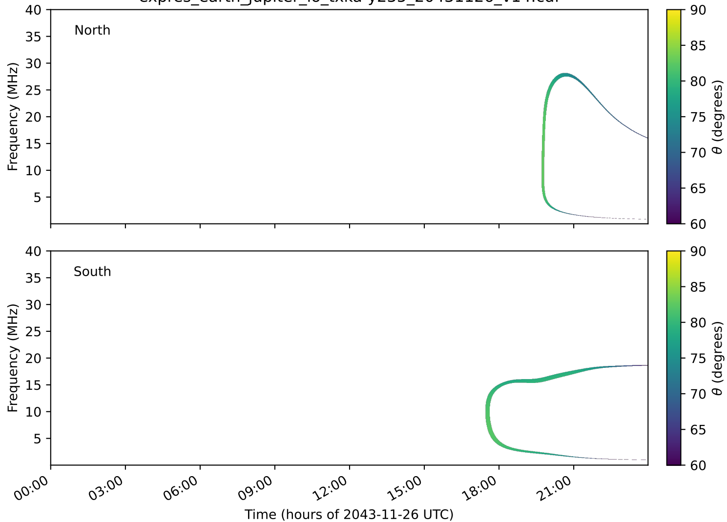
expres_earth_jupiter_io_txka-y235_20431126_v14.cdf
