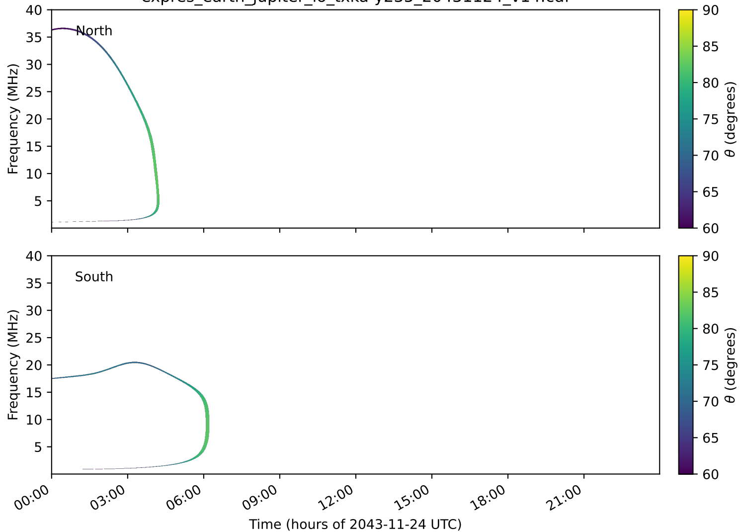
expres_earth_jupiter_io_txka-y235_20431124_v14.cdf
