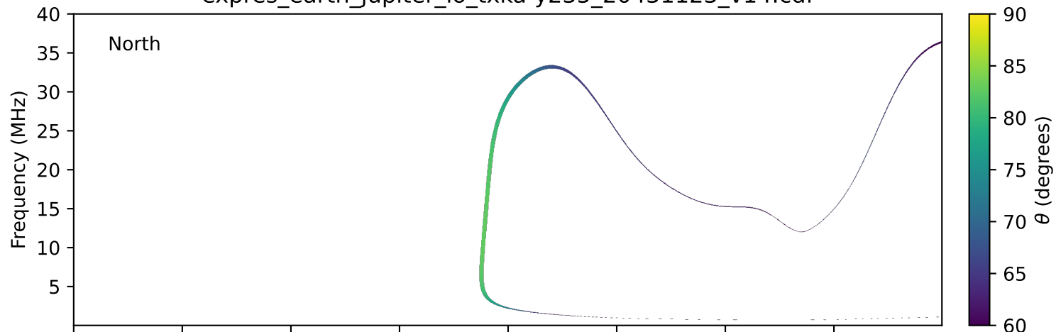
expres_earth_jupiter_io_txka-y235_20431123_v14.cdf
