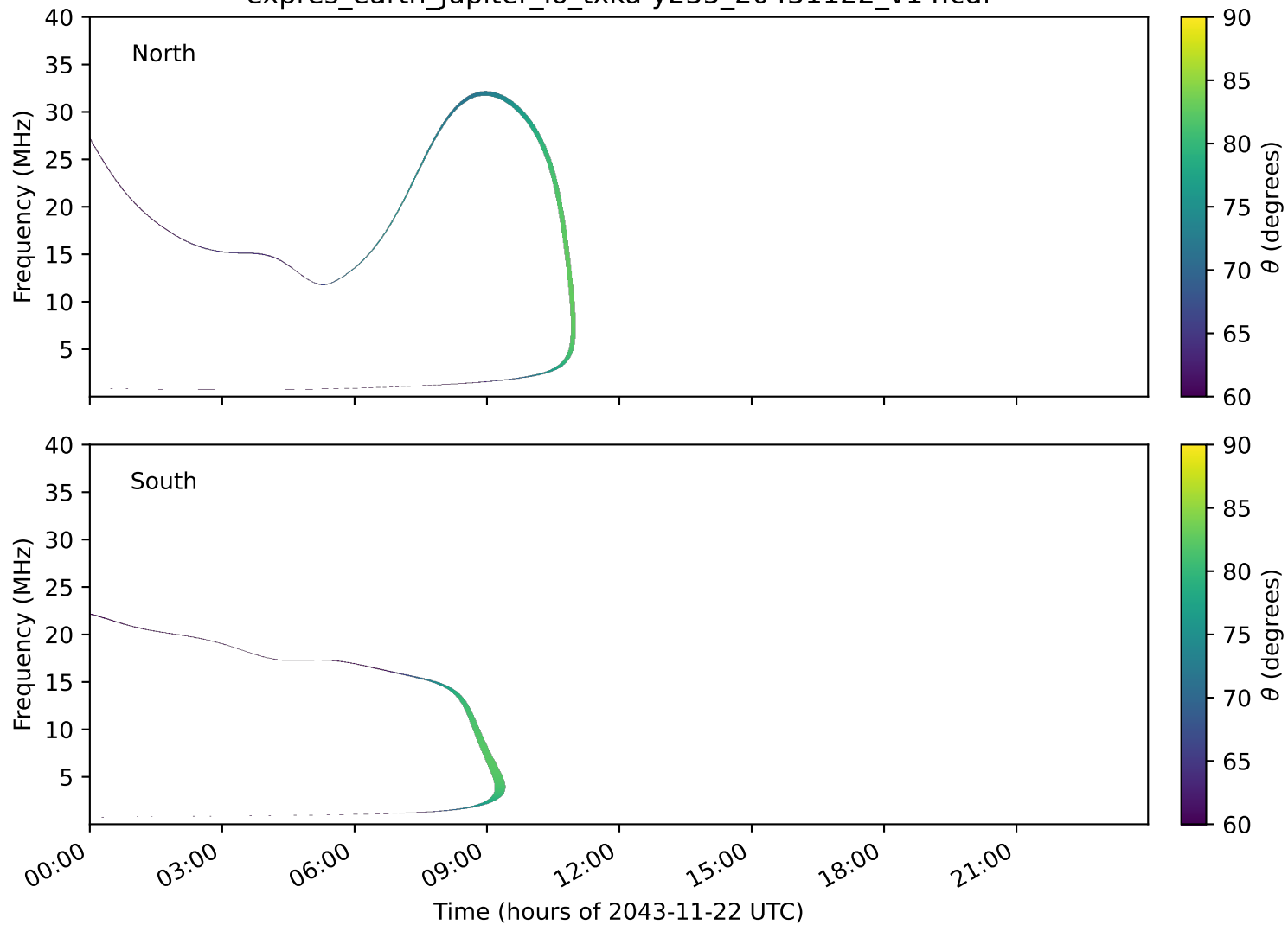
expres_earth_jupiter_io_txka-y235_20431122_v14.cdf
