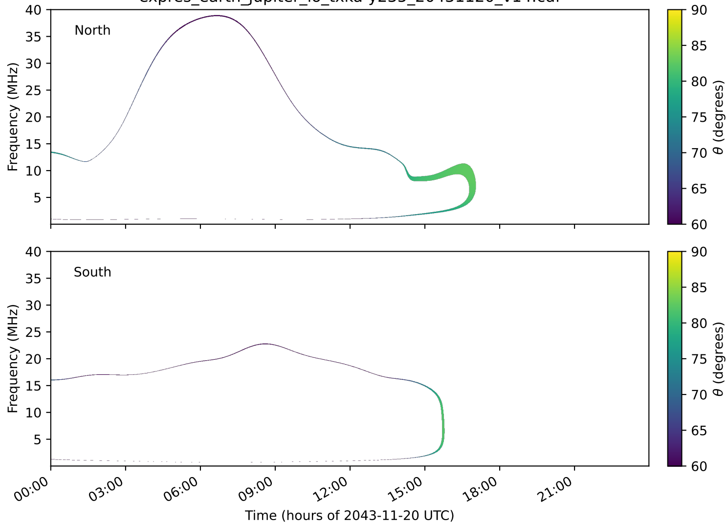
expres_earth_jupiter_io_txka-y235_20431120_v14.cdf
