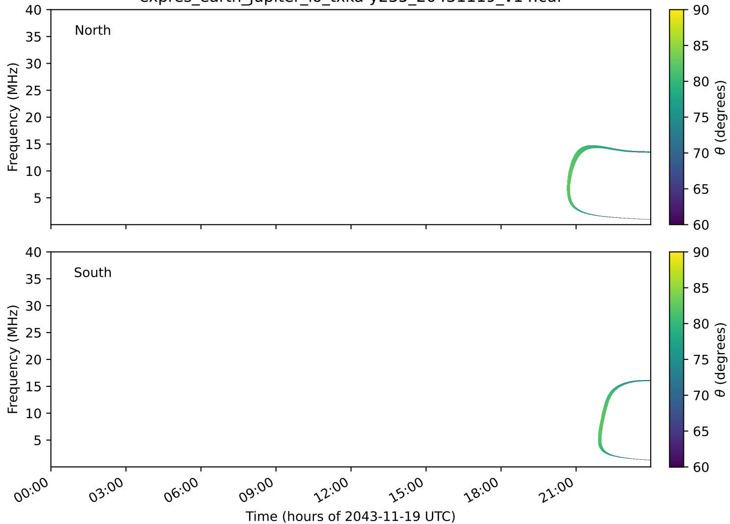
expres_earth_jupiter_io_txka-y235_20431119_v14.cdf
