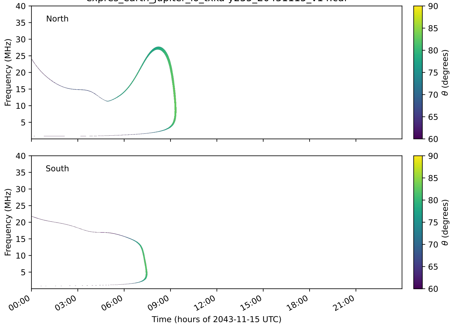
expres_earth_jupiter_io_txka-y235_20431115_v14.cdf
