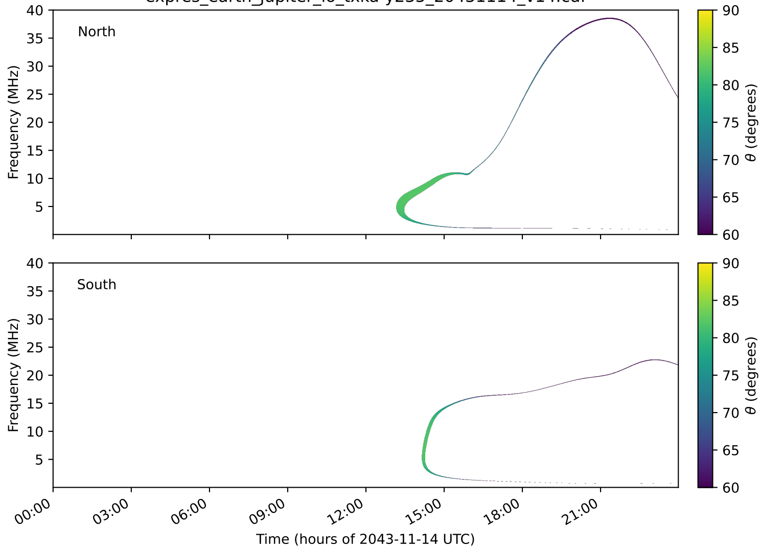
expres_earth_jupiter_io_txka-y235_20431114_v14.cdf
