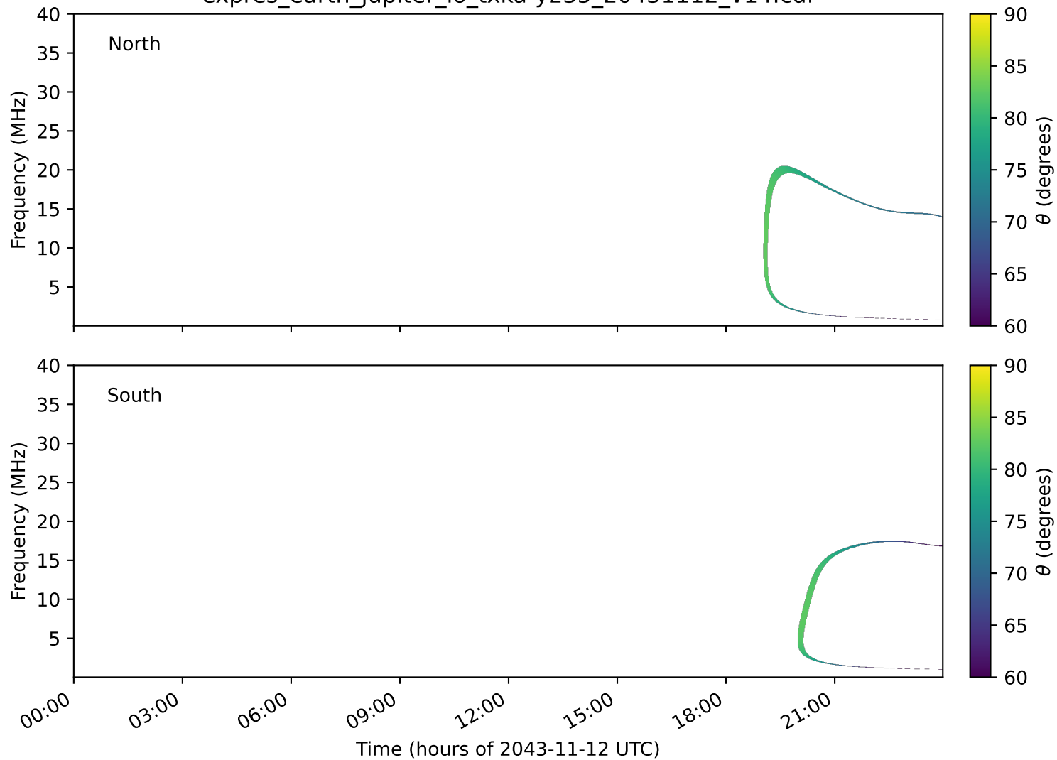
expres_earth_jupiter_io_txka-y235_20431112_v14.cdf
