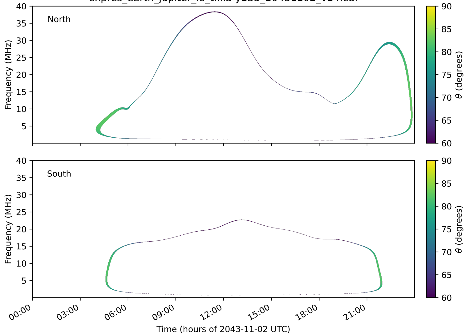
expres_earth_jupiter_io_txka-y235_20431102_v14.cdf
