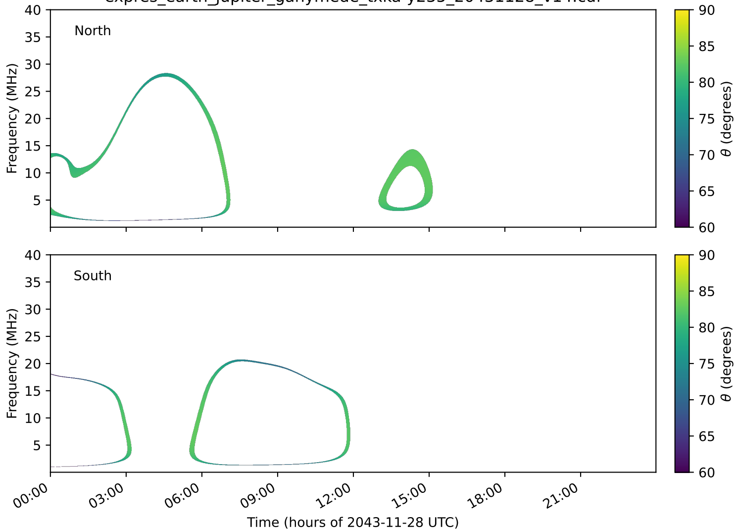
expres_earth_jupiter_ganymede_txka-y235_20431128_v14.cdf
