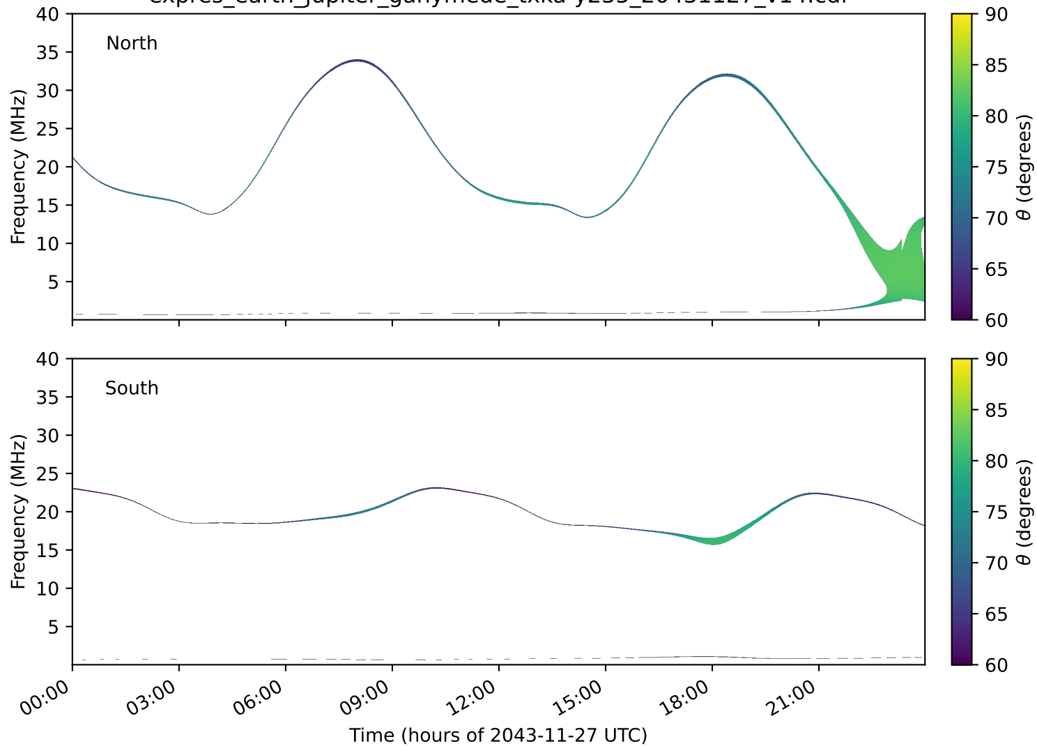
expres_earth_jupiter_ganymede_txka-y235_20431127_v14.cdf
