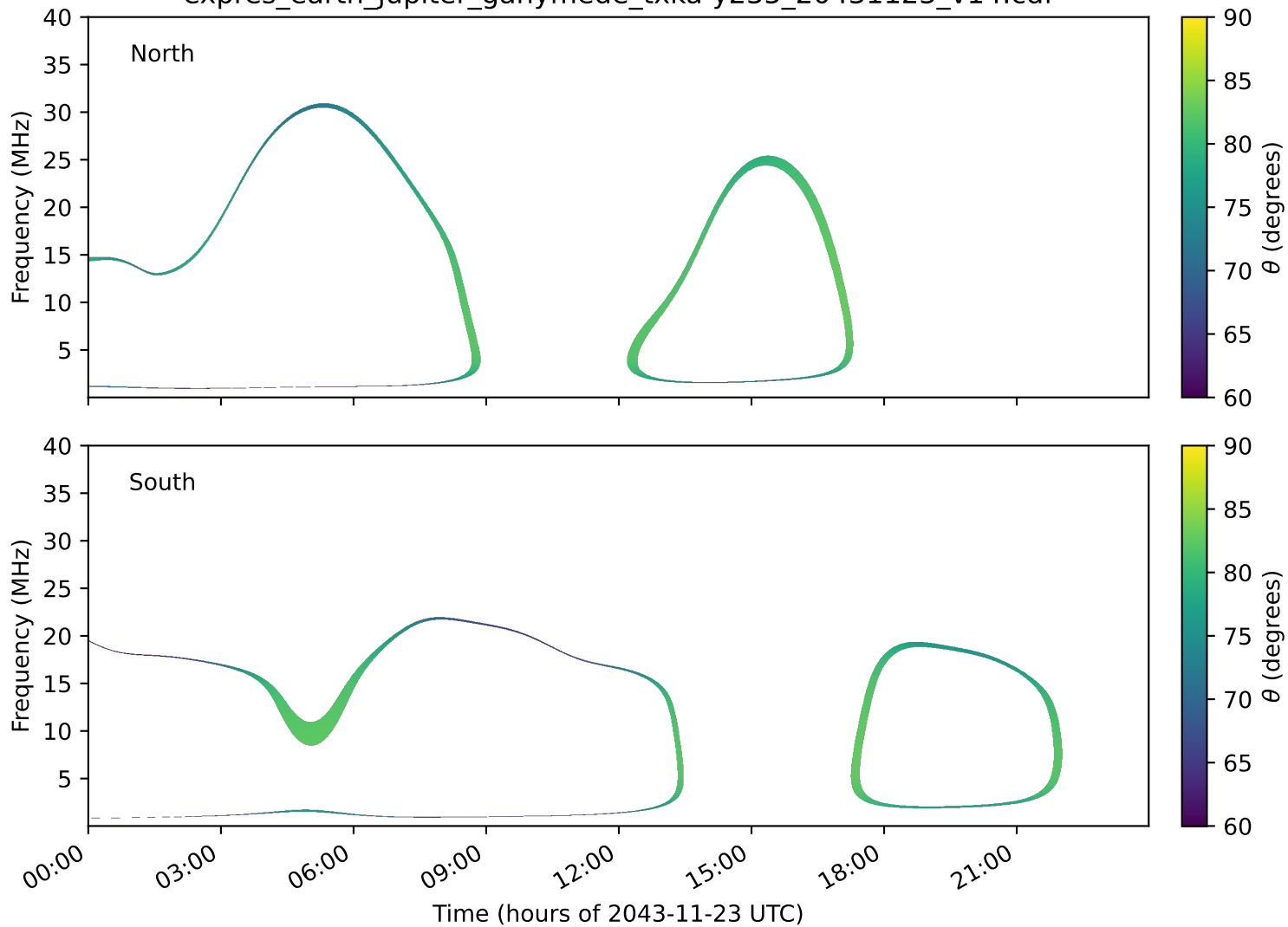
expres_earth_jupiter_ganymede_txka-y235_20431123_v14.cdf
