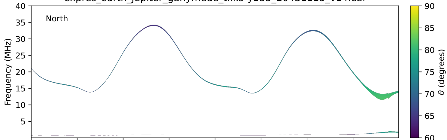
expres_earth_jupiter_ganymede_txka-y235_20431115_v14.cdf
