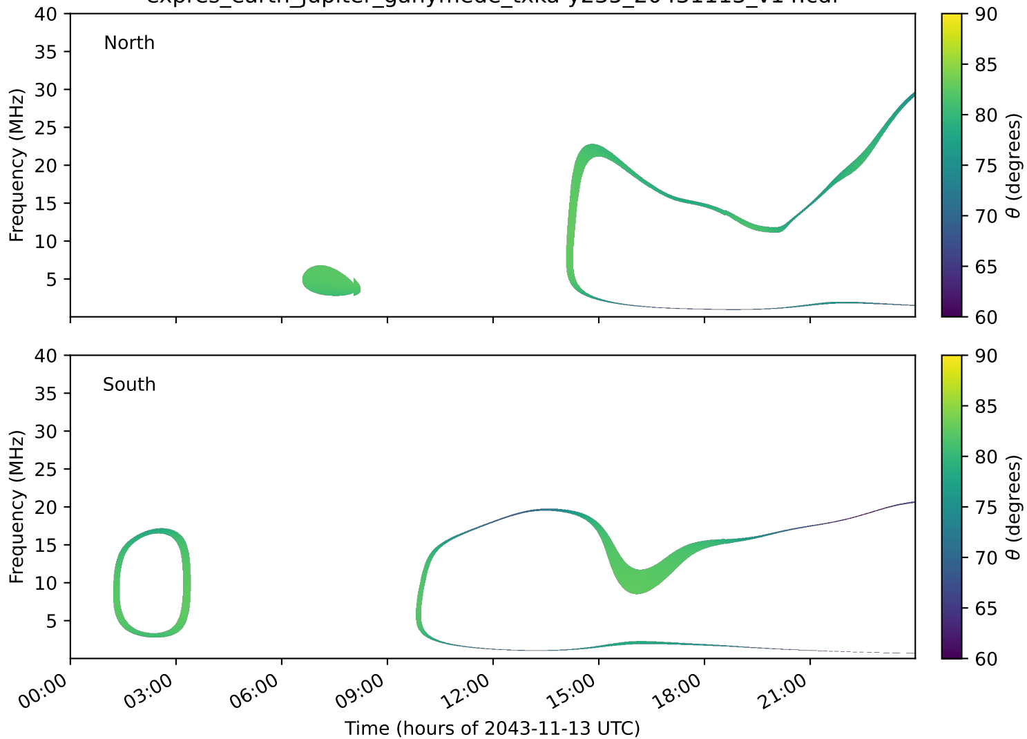
expres_earth_jupiter_ganymede_txka-y235_20431113_v14.cdf
