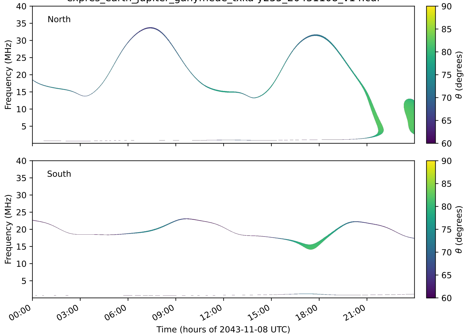
expres_earth_jupiter_ganymede_txka-y235_20431108_v14.cdf
