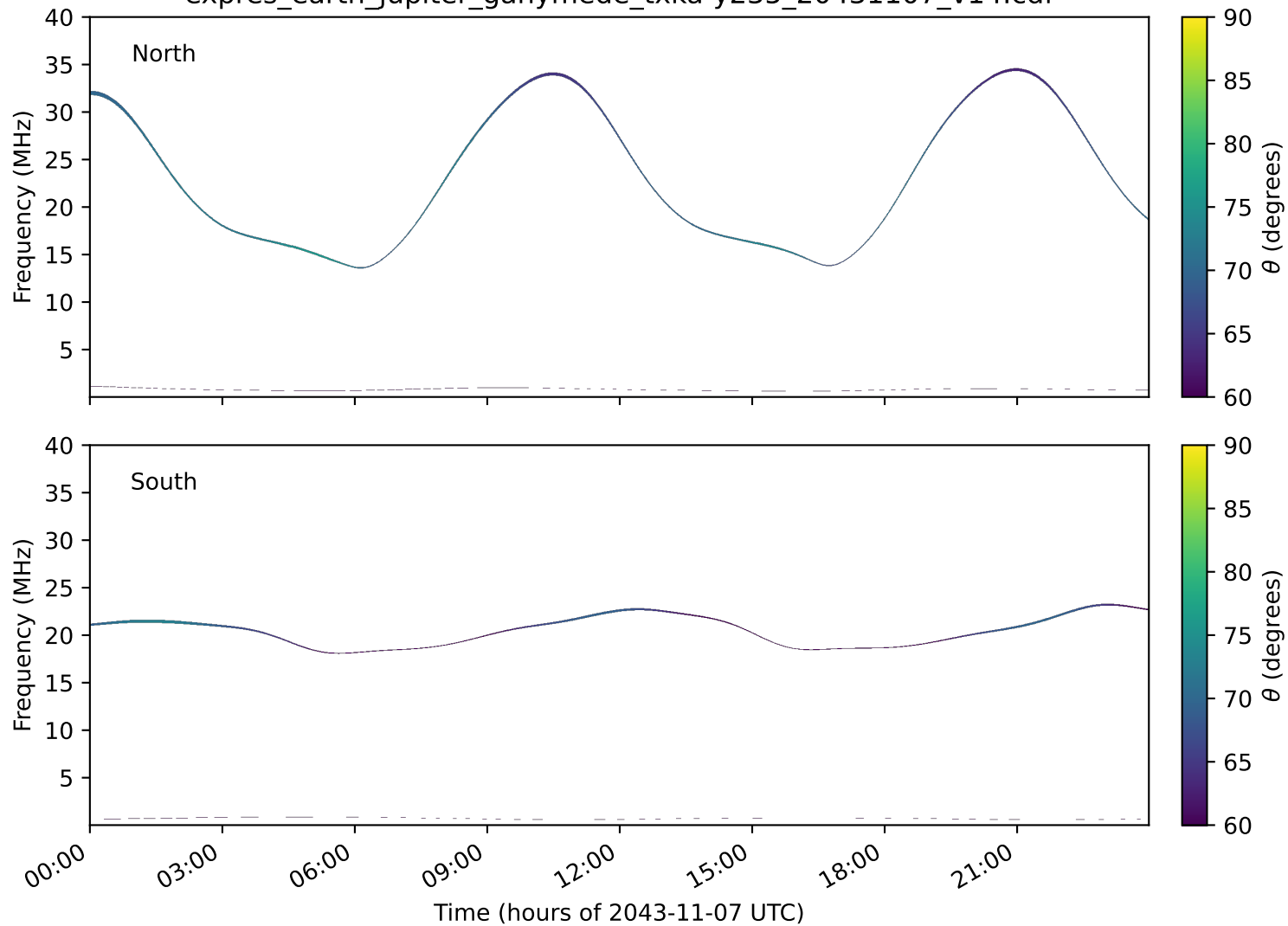
expres_earth_jupiter_ganymede_txka-y235_20431107_v14.cdf
