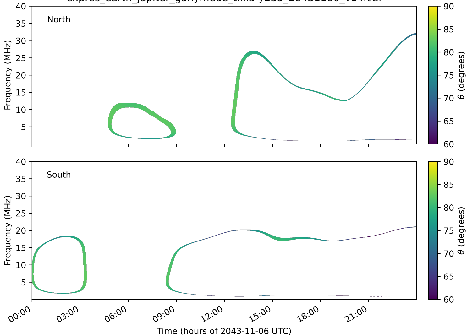
expres_earth_jupiter_ganymede_txka-y235_20431106_v14.cdf
