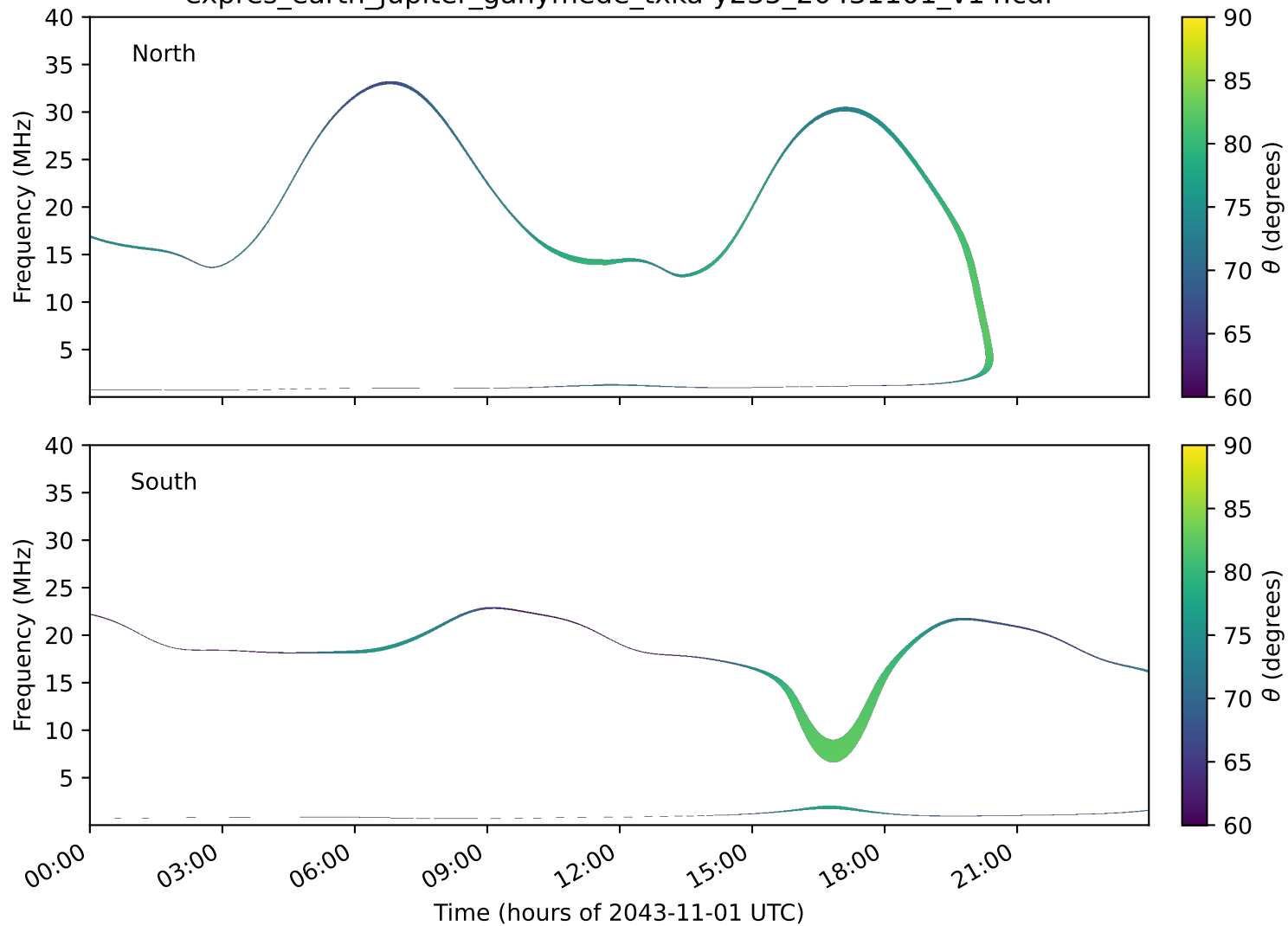
expres_earth_jupiter_ganymede_txka-y235_20431101_v14.cdf
