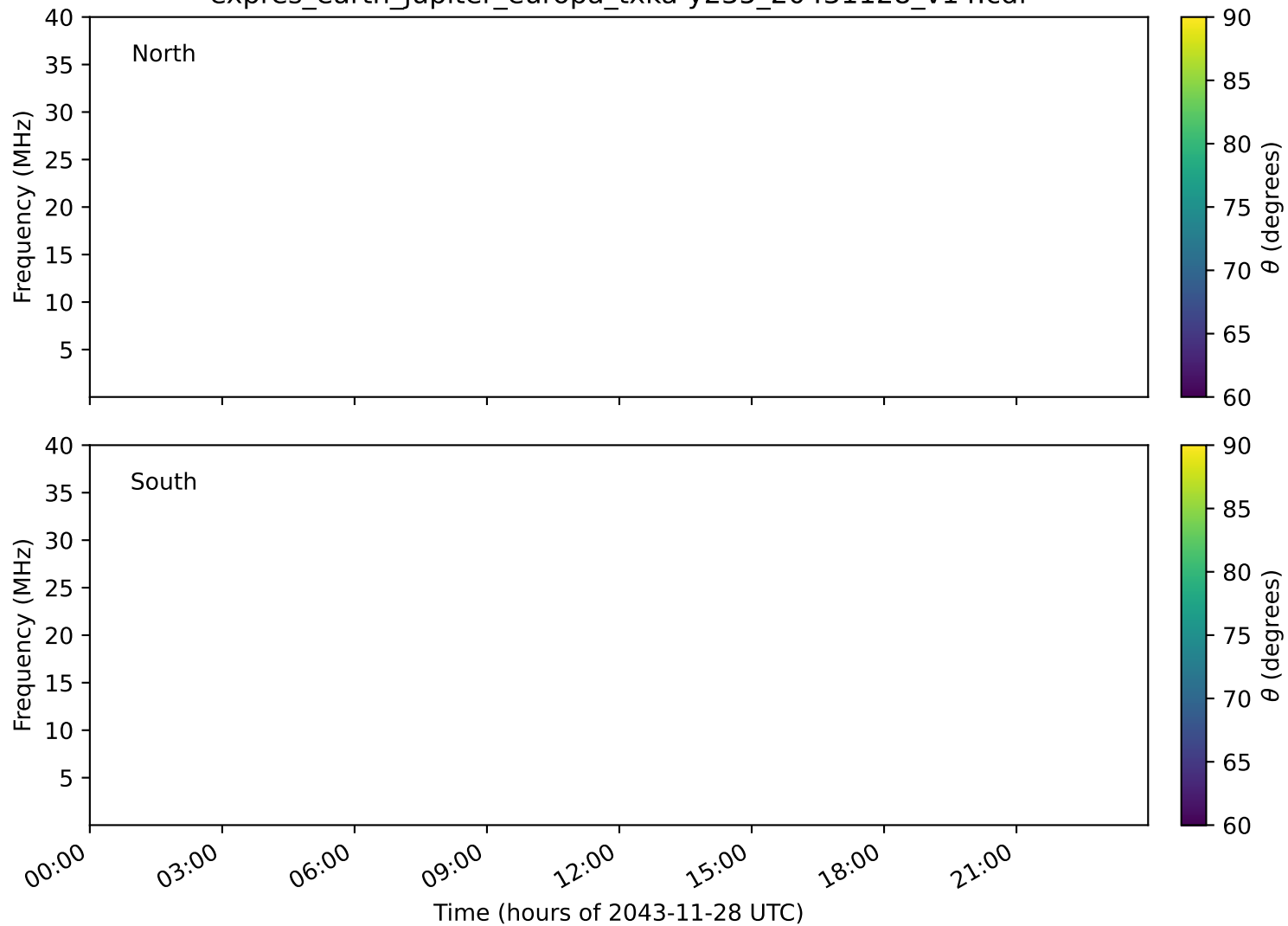
expres_earth_jupiter_europa_txka-y235_20431128_v14.cdf
