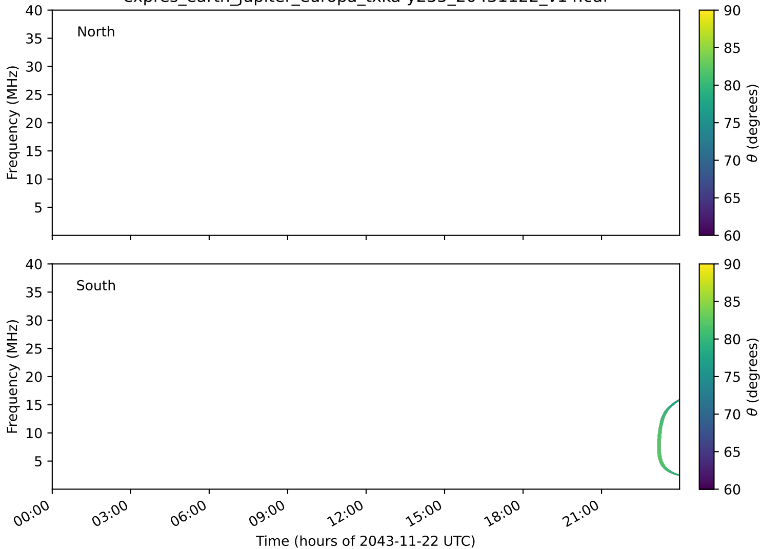
expres_earth_jupiter_europa_txka-y235_20431122_v14.cdf
