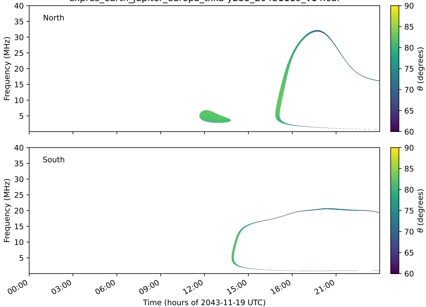
expres_earth_jupiter_europa_txka-y235_20431119_v14.cdf
