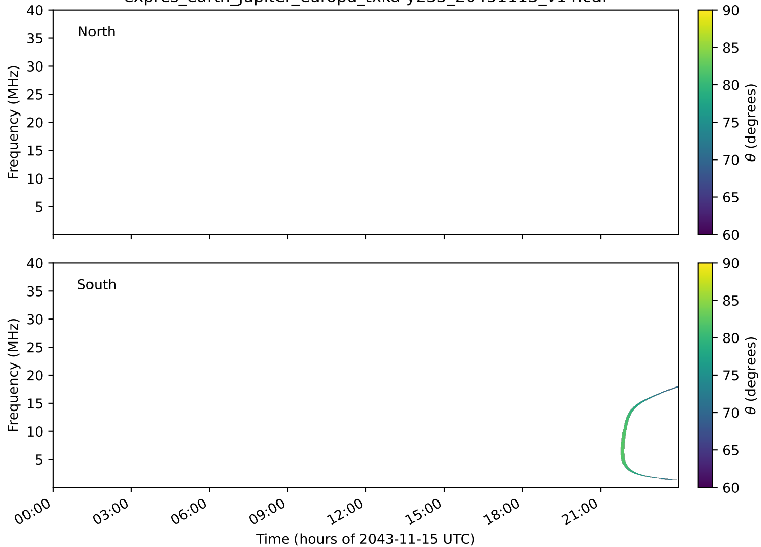
expres_earth_jupiter_europa_txka-y235_20431115_v14.cdf
