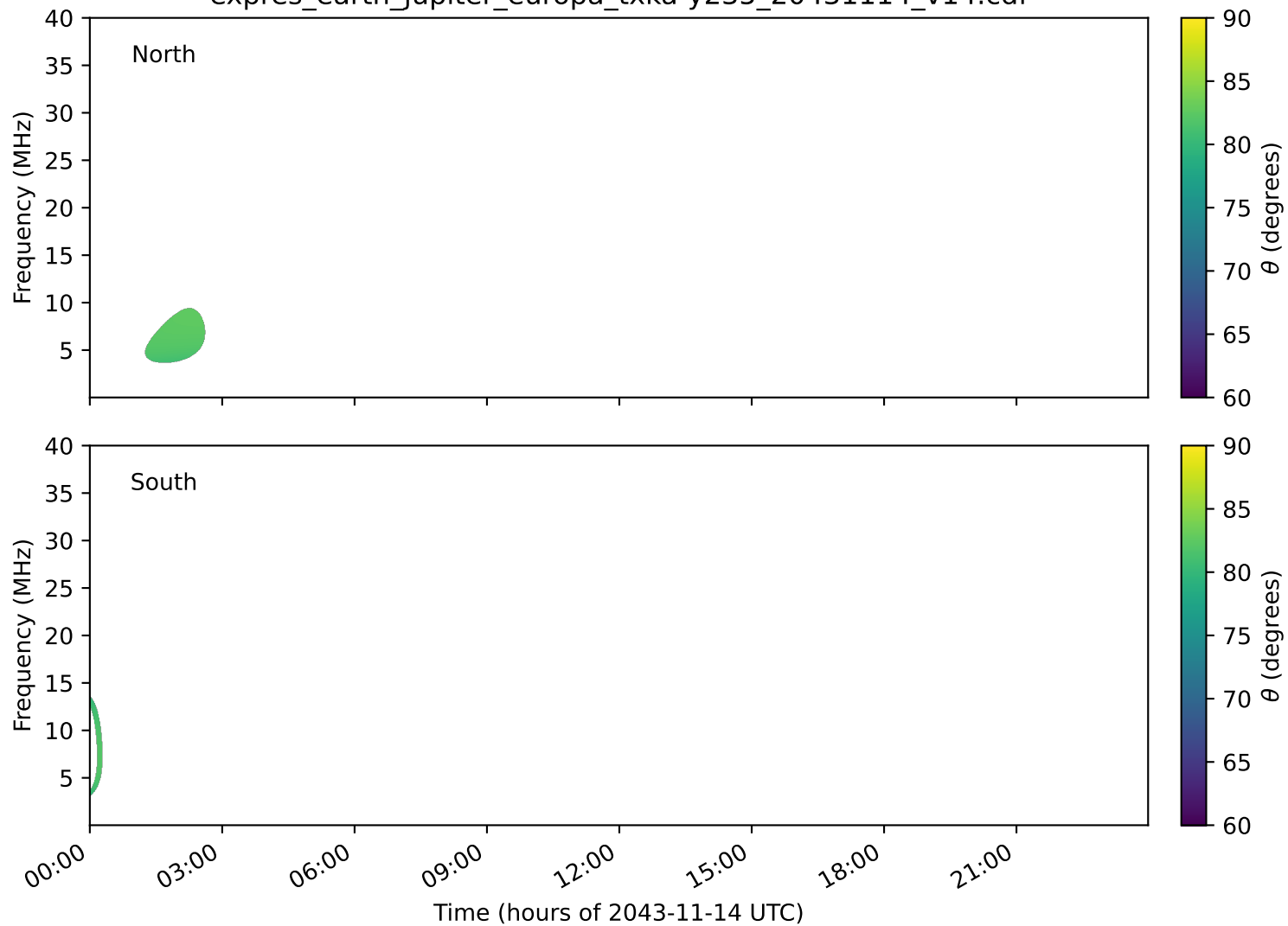
expres_earth_jupiter_europa_txka-y235_20431114_v14.cdf
