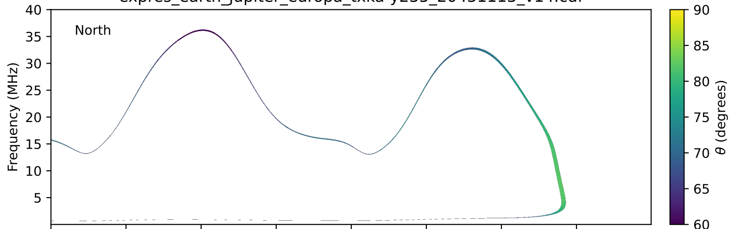
expres_earth_jupiter_europa_txka-y235_20431113_v14.cdf
