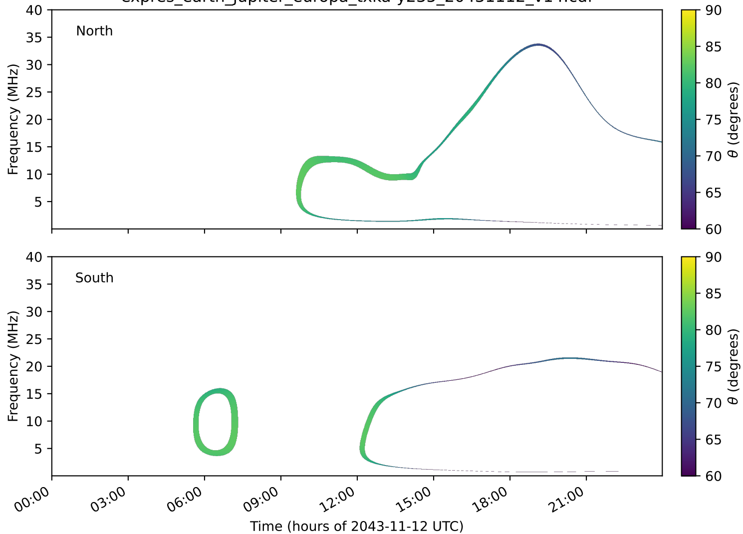
expres_earth_jupiter_europa_txka-y235_20431112_v14.cdf
