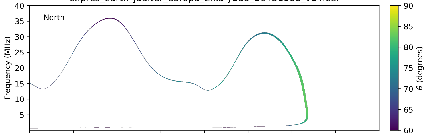
expres_earth_jupiter_europa_txka-y235_20431106_v14.cdf
