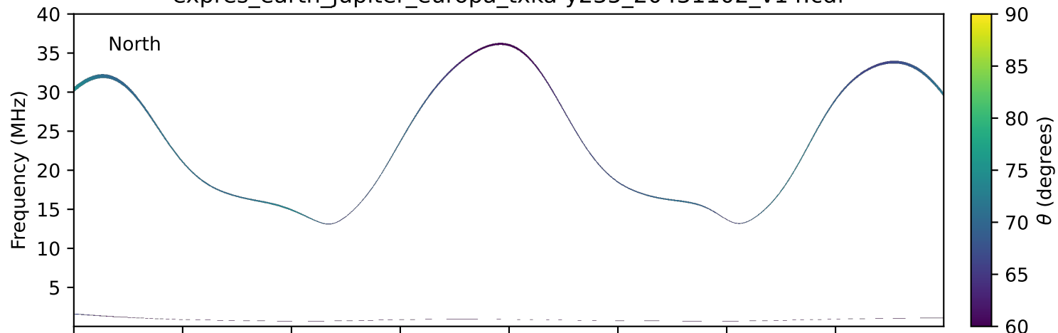
expres_earth_jupiter_europa_txka-y235_20431102_v14.cdf
