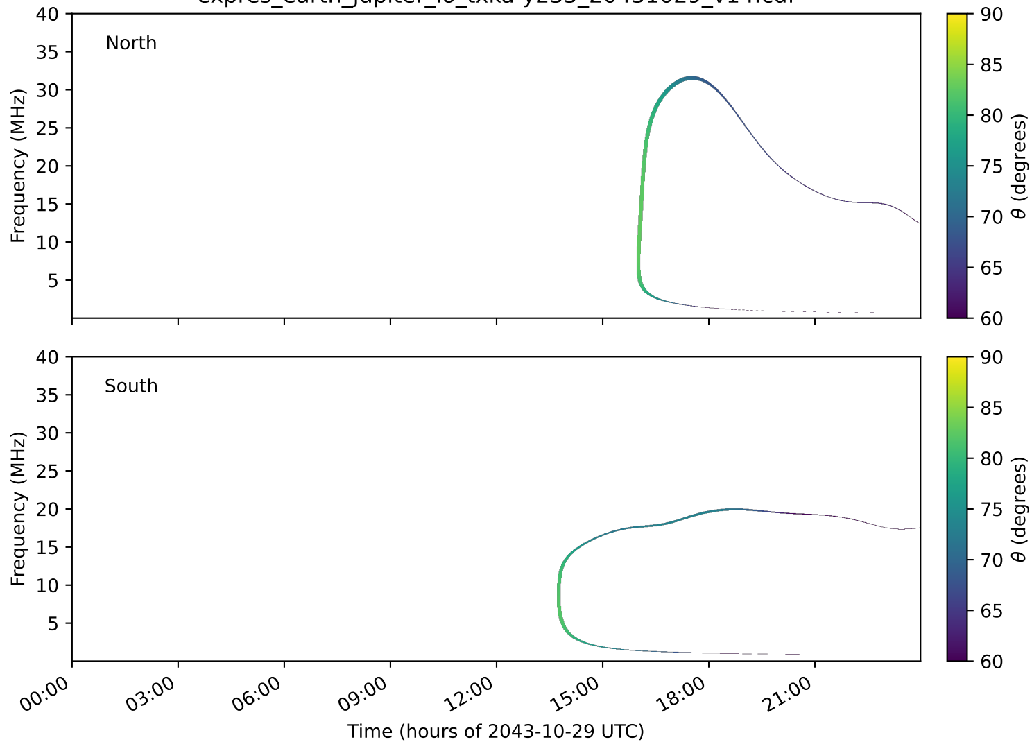
expres_earth_jupiter_io_txka-y235_20431029_v14.cdf
