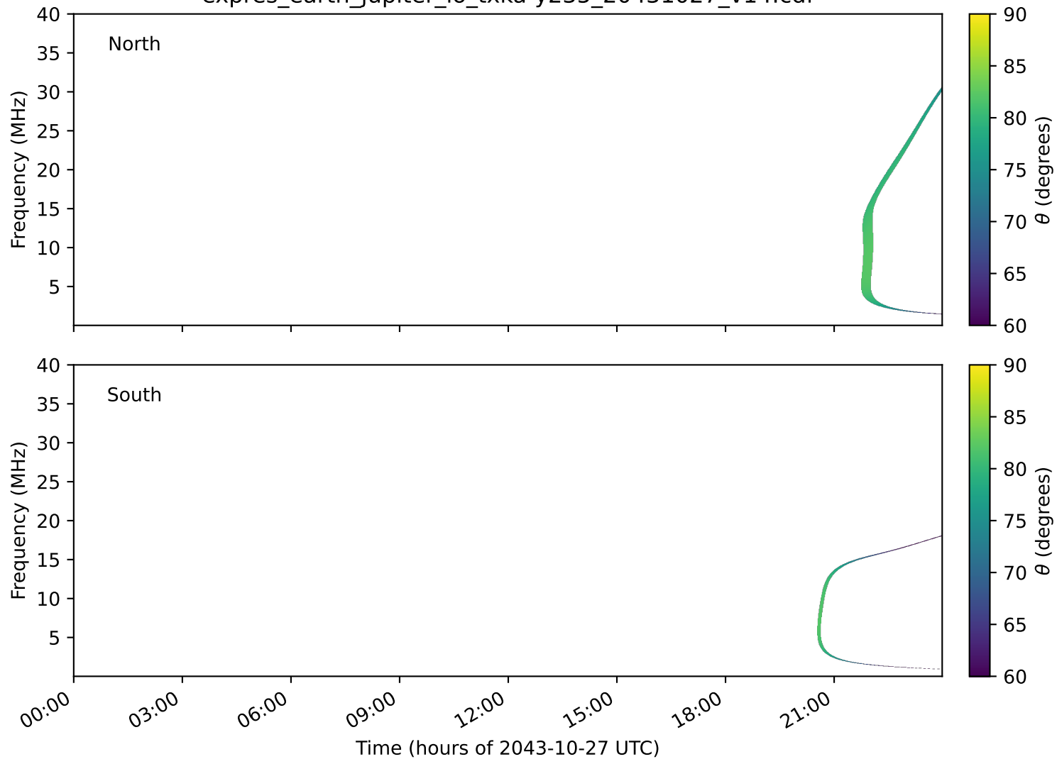
expres_earth_jupiter_io_txka-y235_20431027_v14.cdf
