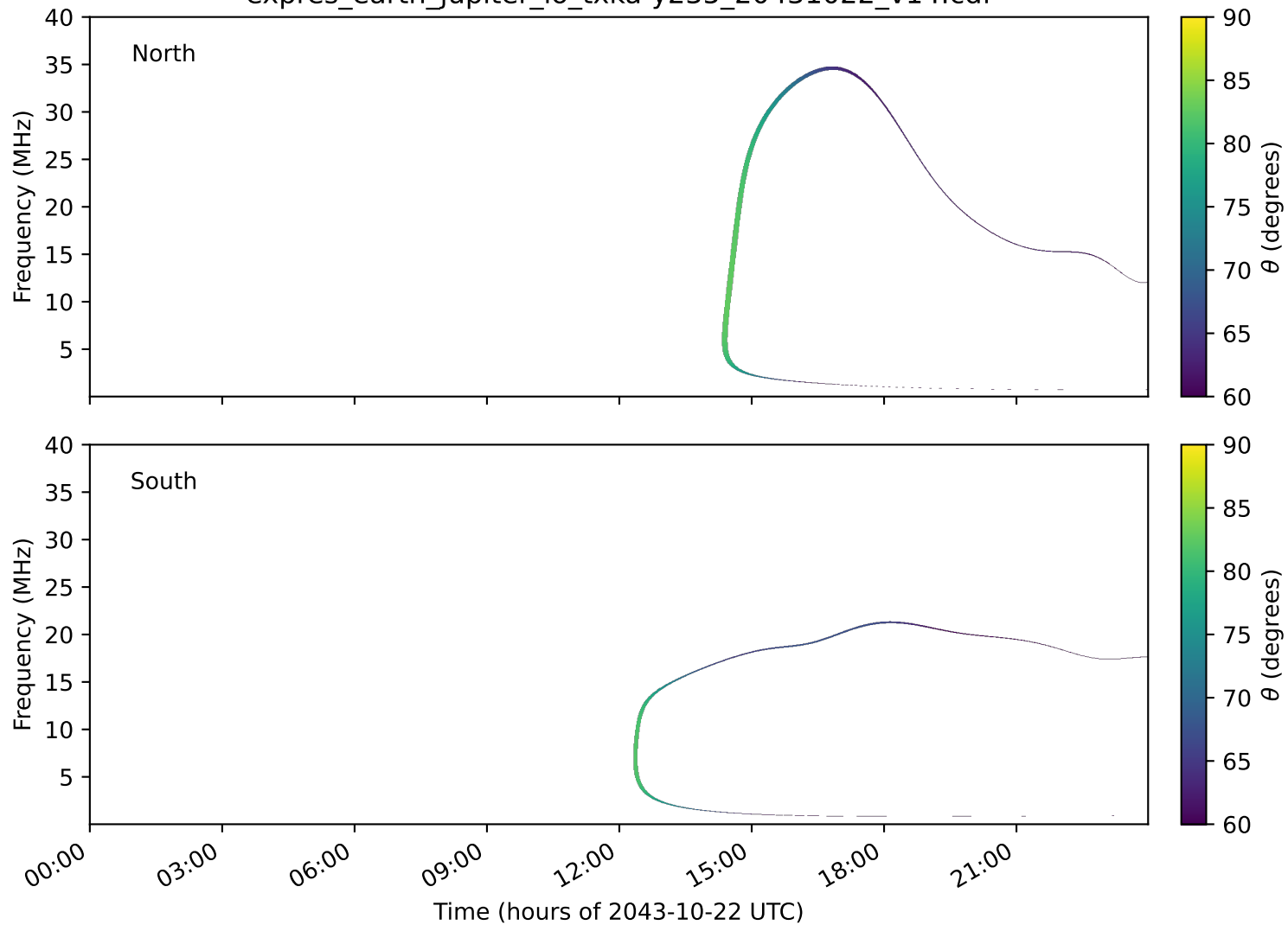
expres_earth_jupiter_io_txka-y235_20431022_v14.cdf
